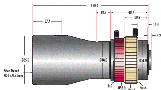
0.5X & 0.36X Telecentric Lenses
