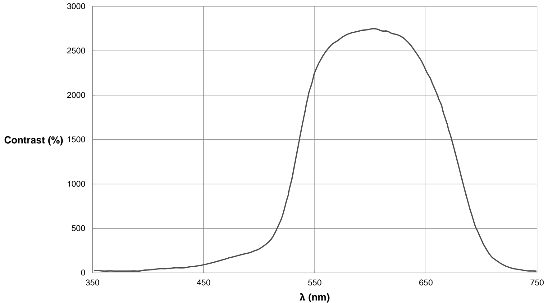
Machine Vision Linear Polarizer, 3000:1 (400nm-700nm) FOR REFERENCE ONLY
