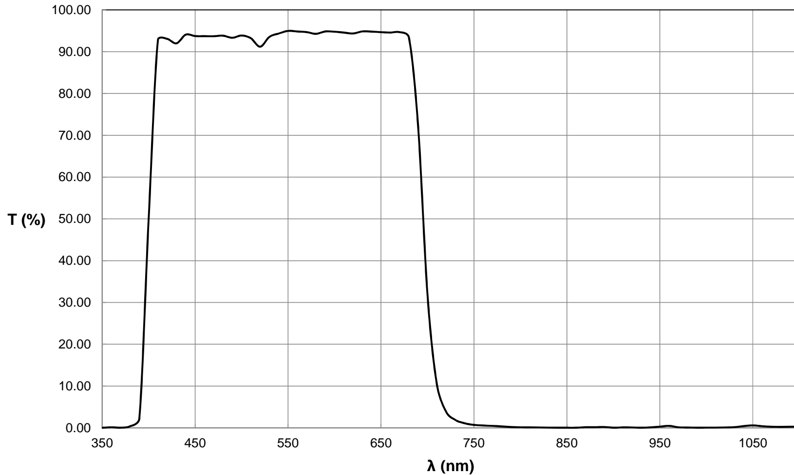
Near-IR/UV Block Machine Vision Bandpass Filter, 550nm FOR REFERENCE ONLY
